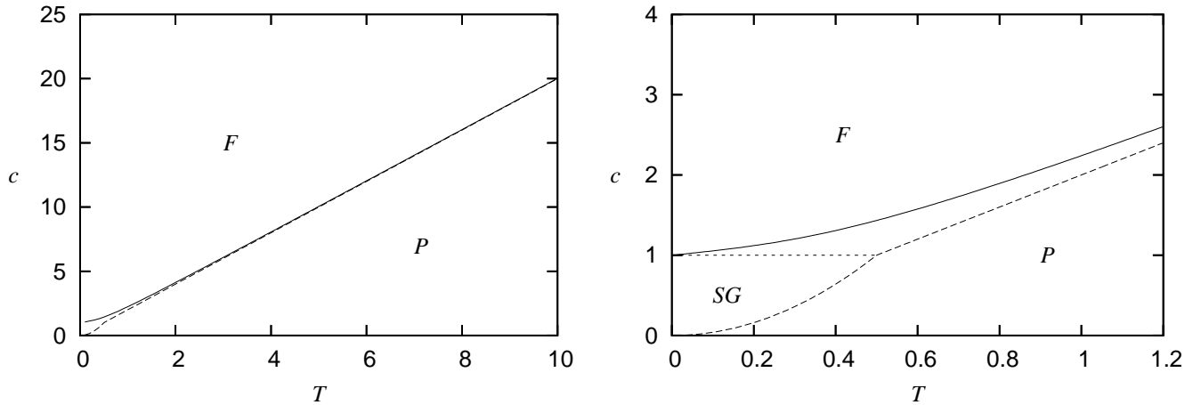
FIG. 1: Phase diagram in T - c plane. Solid curve: sparse model (Model ER), dotted curve: fully connected model (Model FC). Right panel: Enlargement of the left panel.
