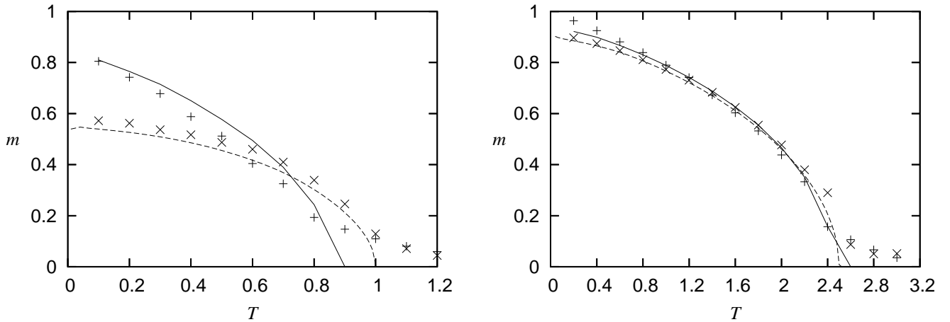
FIG. 2: T dependence of m . Left panel: c = 2 , right panel: c = 5 . Curves: theoretical results. Symbols: numerical results of the Langavini eq.(1) for N = 2000 . Solid curve and + : sparse model (Model ER), dashed curve and x: fully connected model (Model FC).
